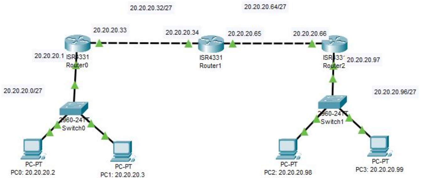
Fig: Topology of The Network
